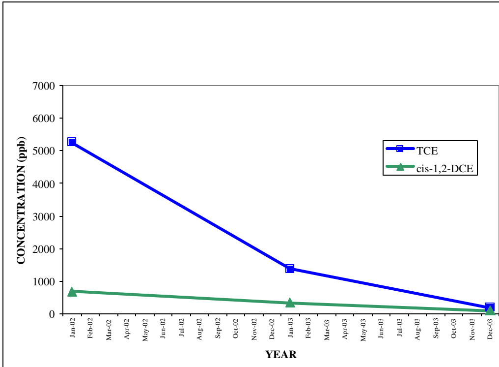
FIGURE 2. PTW-1 TCE and cis-1,2-DCE concentration Jan 2002 (prior to full-scale ARD) – Dec 2003
