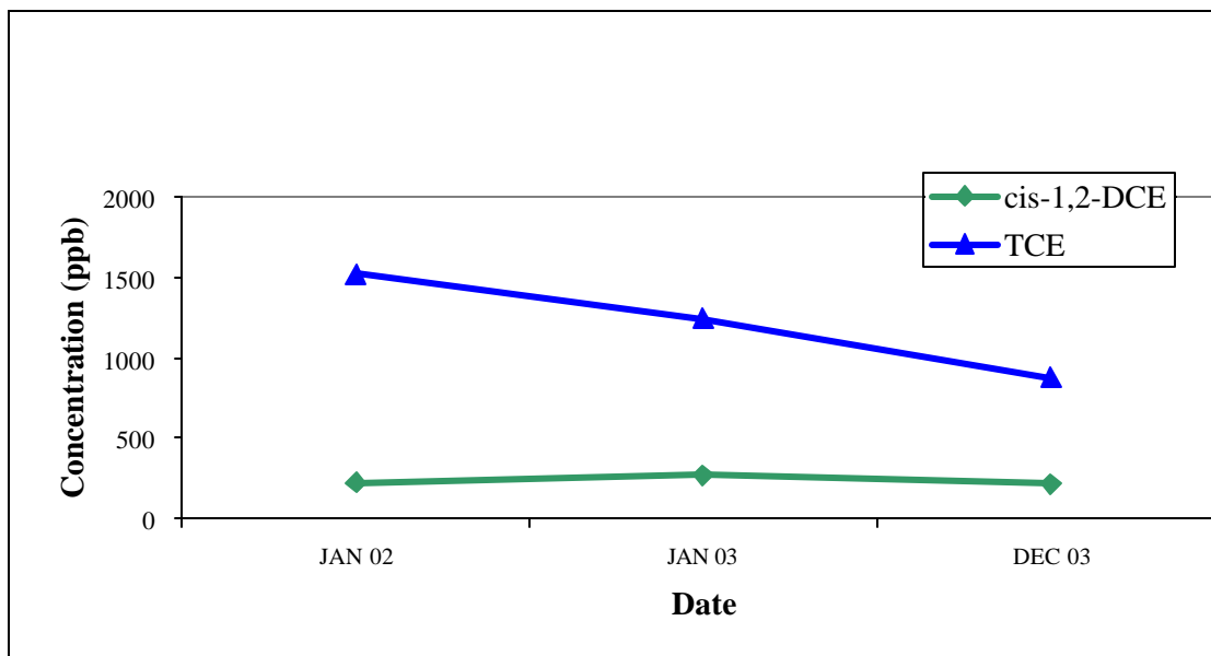
FIGURE 3. Site-wide average TCE and cis-1,2-DCE concentration Jan 2002 (prior to full scale ARD) – Dec 2003
